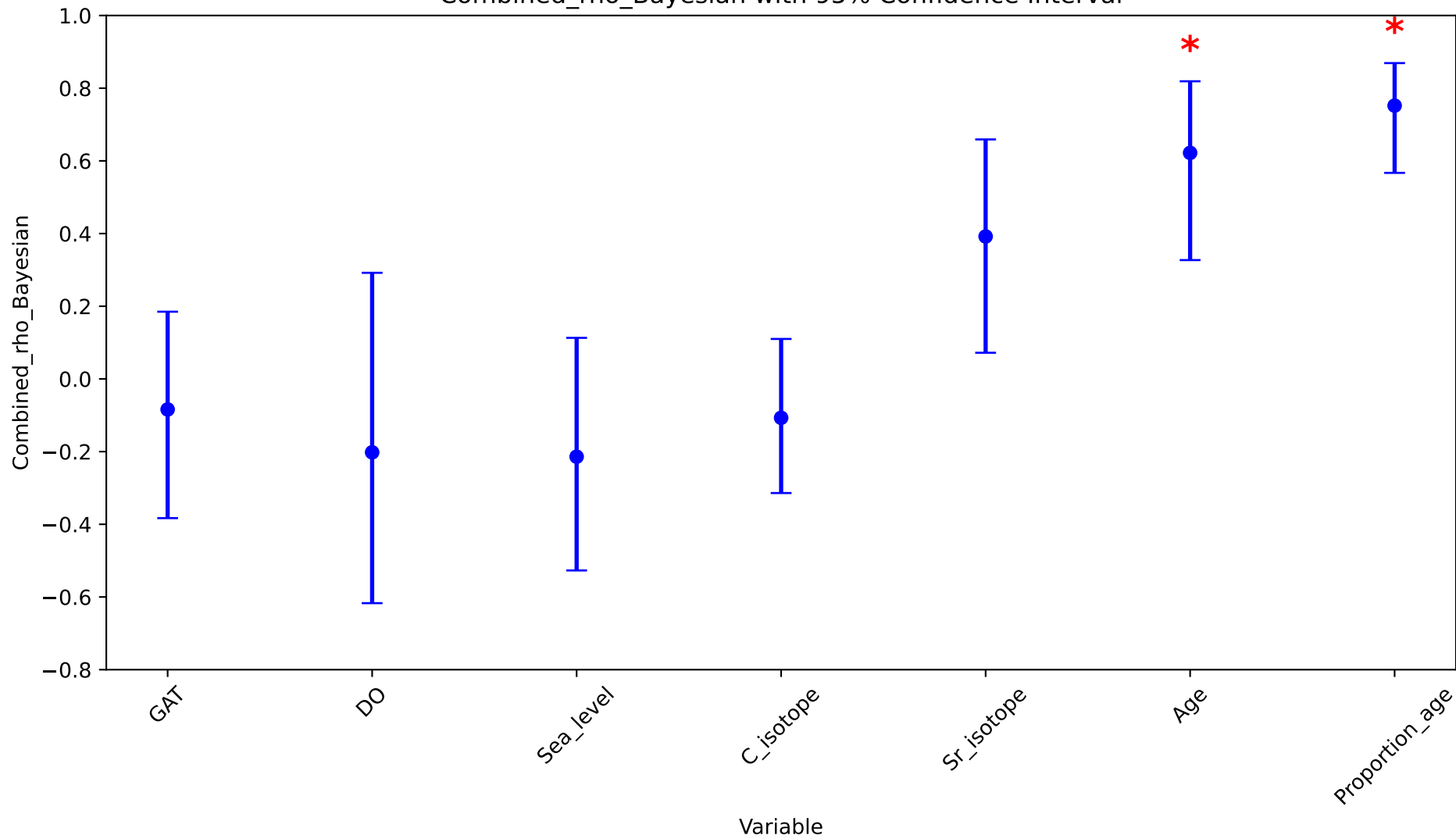
Combined_rho_Bayesian with 95% Confidence Interval
